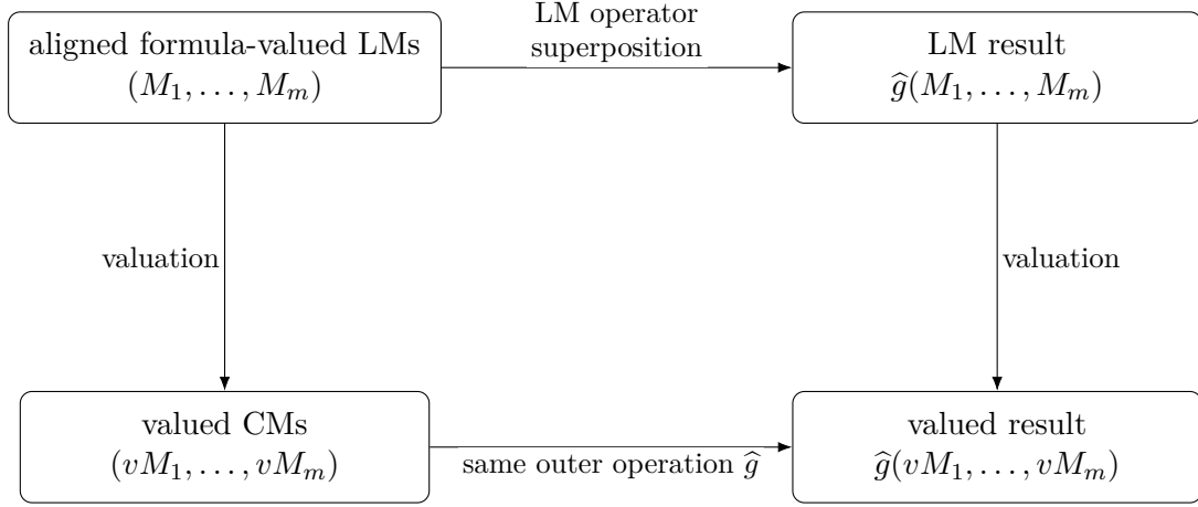
Figure 2: LM-centered coherence under valuation. The same outer Boolean operation may be applied to aligned formula-valued operators before valuation or to their valued CMs afterward. Logical pairing and common input-frame pullbacks satisfy analogous squares because they are Boolean homomorphisms on the pointwise operator algebra.
